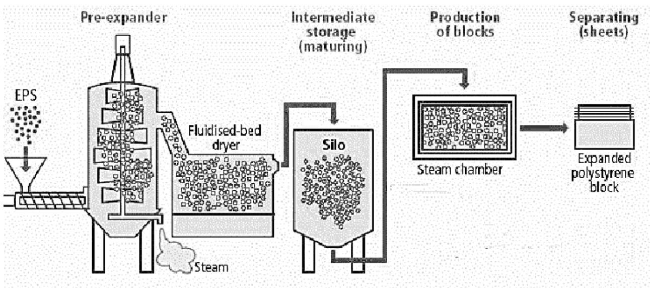
Figure 1. The technological process of an EPS production.
